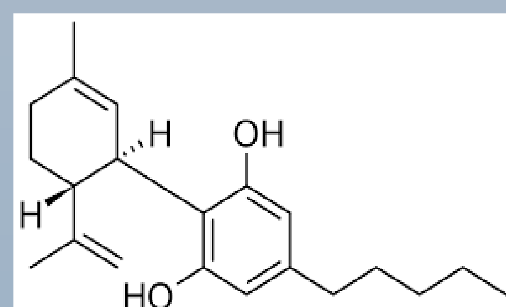
Fig 3. Chemical structure of cannabidiol (CBD).
